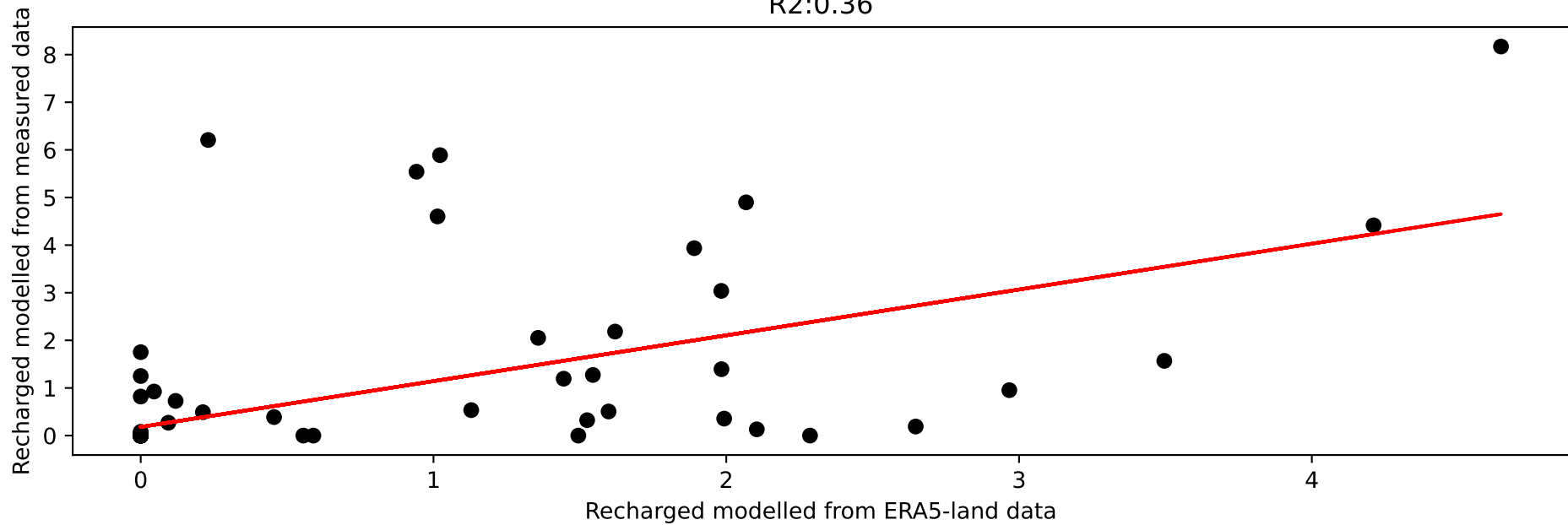
Un-irrigated weekly recharge Function of ERA5 recharge R^2:0.36
