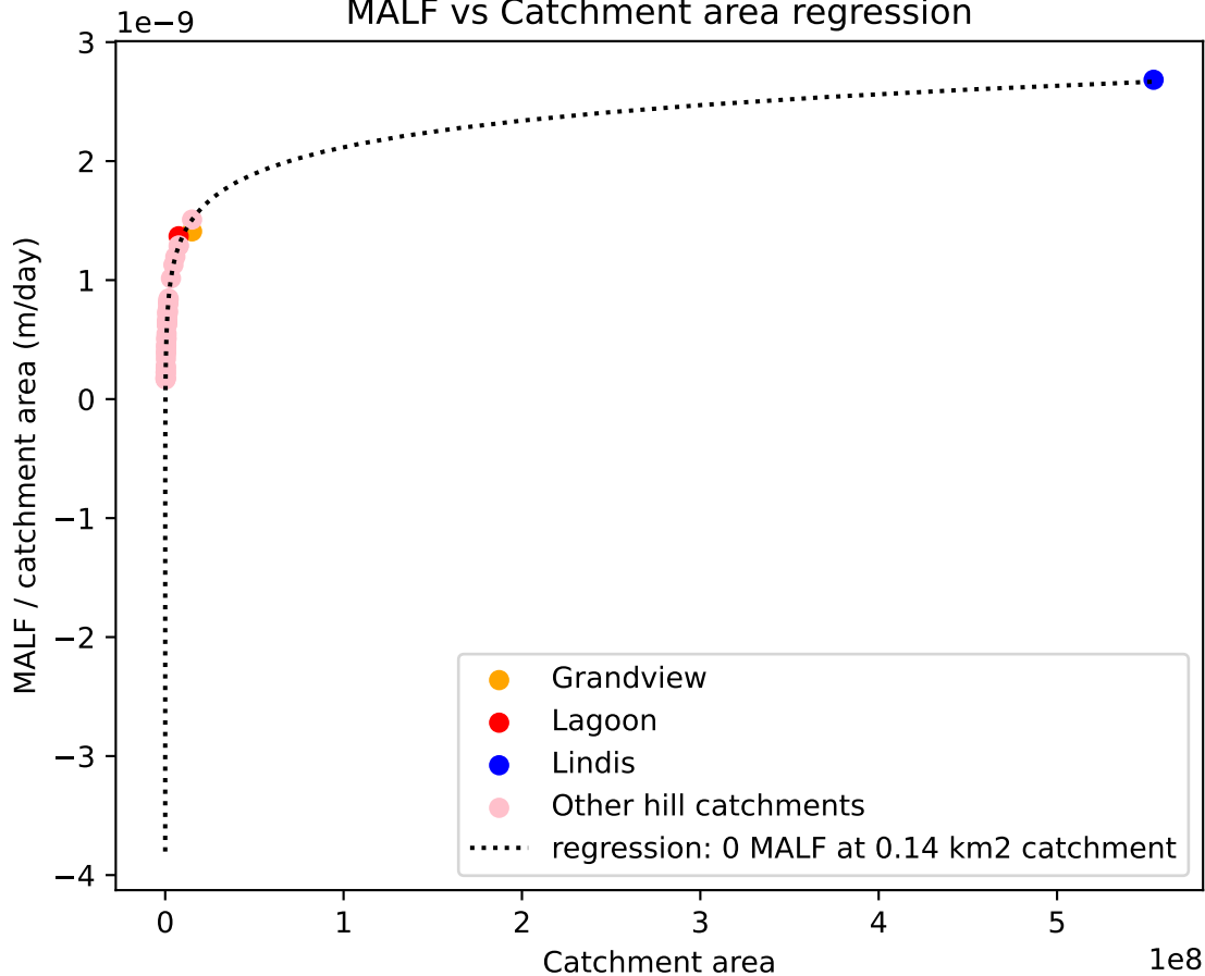
MALF vs Catchment area regression
