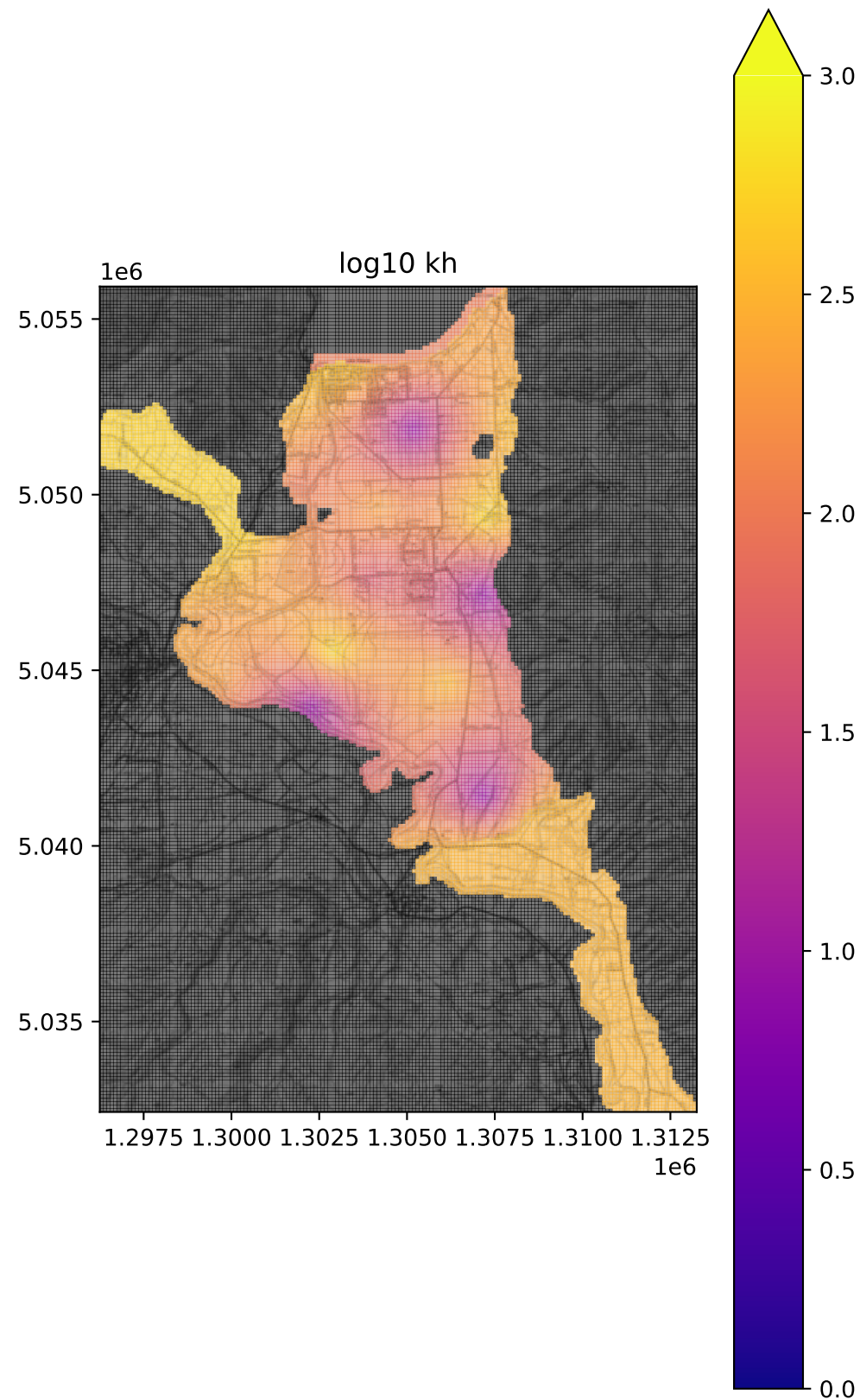
example RBF multiquadric interpolation
