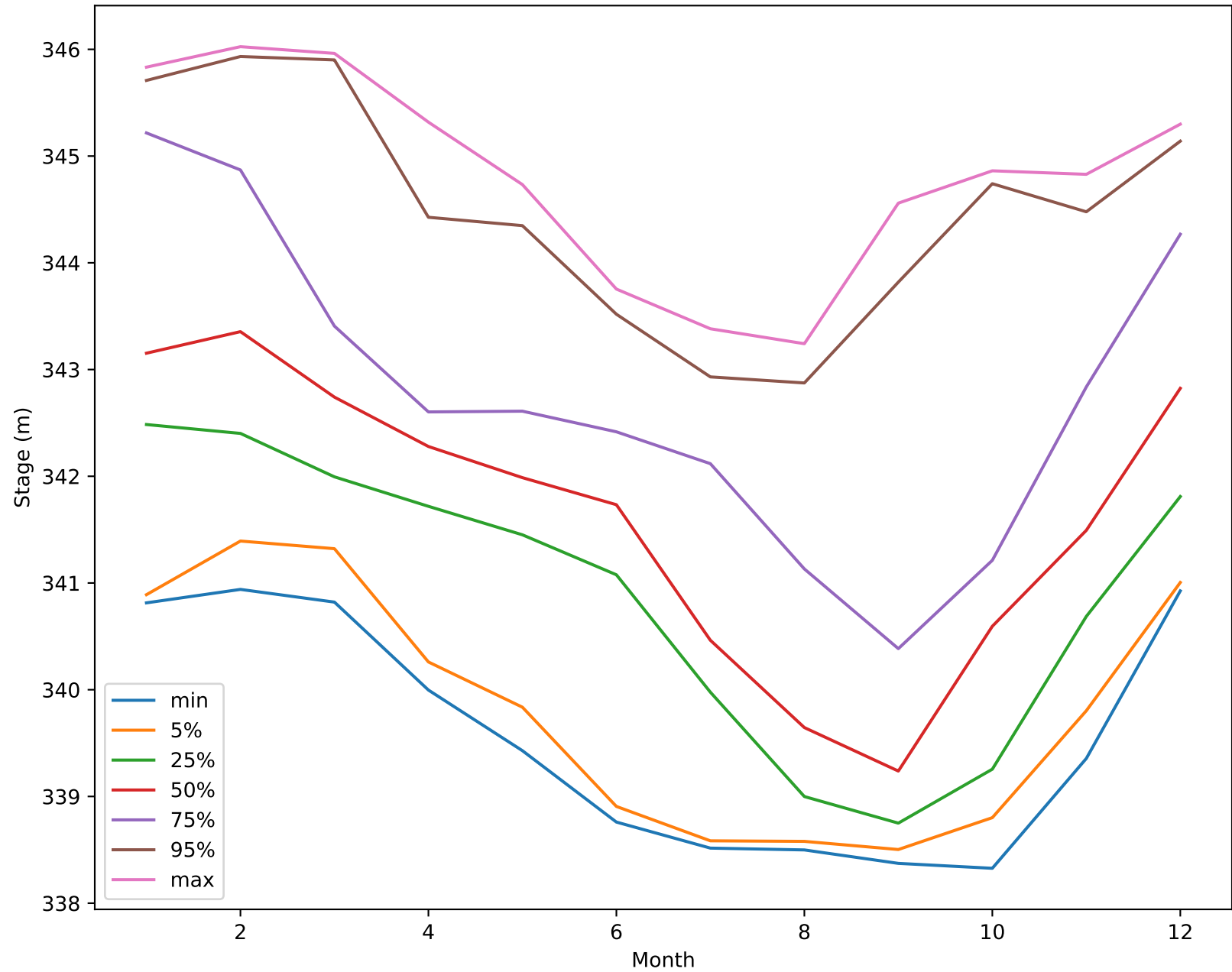
Monthly lake level
