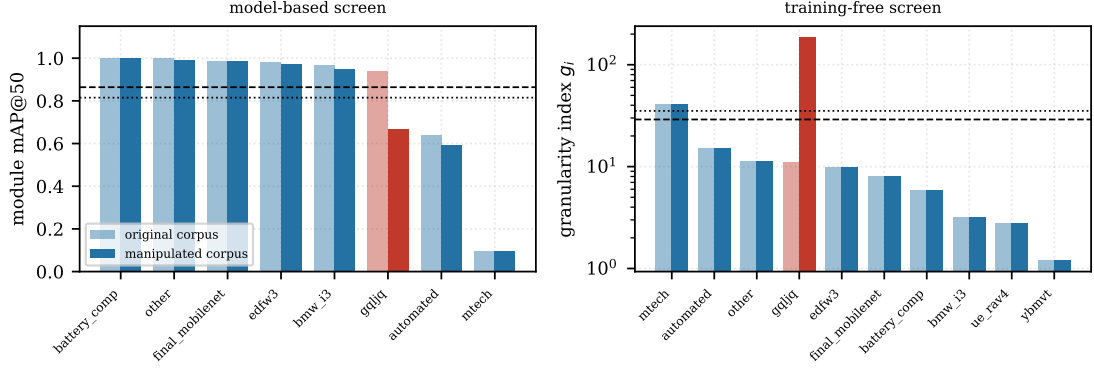
Figure 2: Positive control on both screens. Pale bars are the original corpus, solid bars the corpus in which one consensus source has been relabelled to a sub-component convention. Dashed and dotted lines are the robust fences before and after manipulation. The manipulated source is the only one whose flag status changes.
