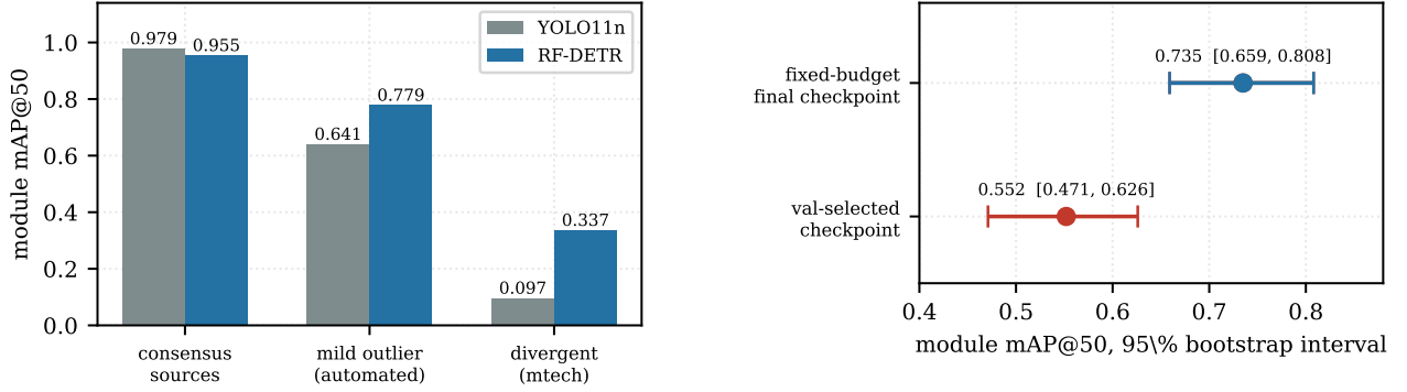
Figure 4: Model selection against single-source validation data. Bars are 95% bootstrap intervals over 500 resamples. The checkpoint chosen by validation accuracy is the worse of the two and the intervals do not overlap.
