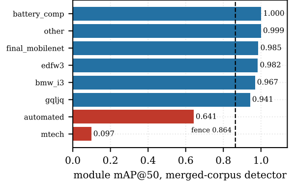
Figure 1: Per-source module accuracy for the merged-corpus detector, with the robust lower fence of Equation 1 at k = 3 . Two sources fall below the fence, one of them by a wide margin.
