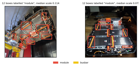
Figure 2: Two frames from the flagged source with their released annotations. Twelve boxes in each carry the label module, every one covering a small internal sub-component; the pack-level modules that every other source annotates are left unmarked. Median normalised module scale is 0.114 and 0.077 respectively, against 0.14 for this source overall and 0.17 to 0.54 across the consensus sources.
