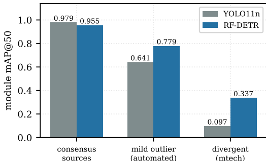
Figure 3: Architecture comparison under a matched budget. The self-supervised pretrained model is marginally weaker on conventionally annotated packs and substantially stronger on both out-of-convention sources.
