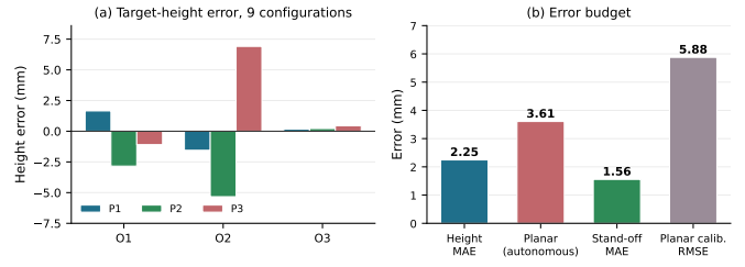
Fig. 2. Localisation on hardware. (a) Signed height error for all nine object-position configurations; O2 dominates the spread. (b) Error budget. The planar figure is the autonomous O1 subset, not the post-alignment measurements.
