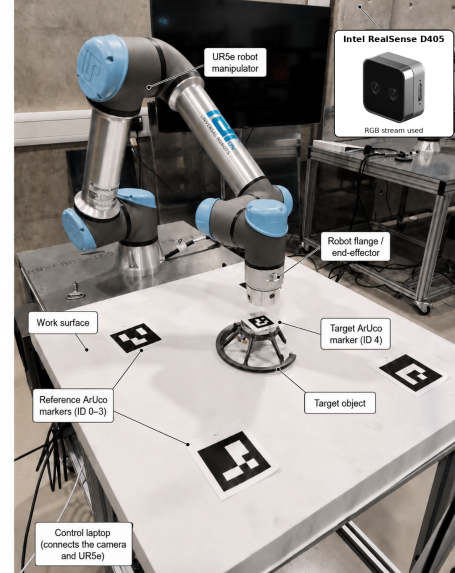
Fig. 3. Vision-guided workcell. An Intel RealSense D405 observes the surface from above; four reference markers bound the workspace and define the Board frame. Only the RGB stream is used. The UR5e approaches the target from above under a bounded two-stage motion.
