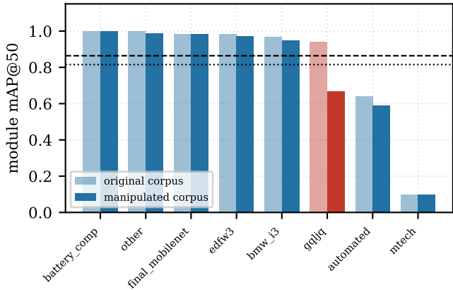
model-based screen
