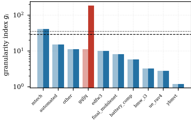
training-free screen
