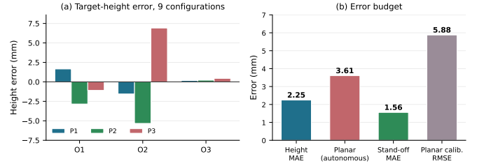
Fig. 2. Localisation on hardware. (a) Signed height error for all nine object-position configurations; O2 dominates the spread. (b) Error budget. The planar figure is the autonomous O1 subset, not the post-alignment measurements.
