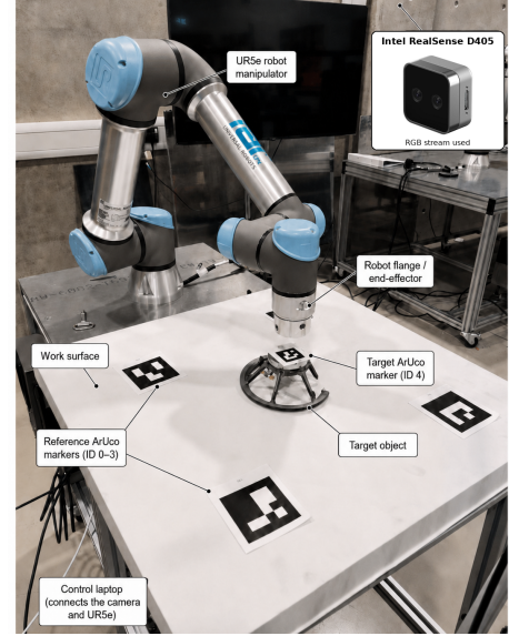
Fig. 3. Vision-guided workcell. An Intel RealSense D405 observes the surface from above; four reference markers bound the workspace and define the Board frame. Only the RGB stream is used. The UR5e approaches the target from above under a bounded two-stage motion.
