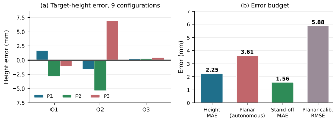
Fig. 1. Localisation on hardware. (a) Signed height error for all nine object-position configurations; O2 dominates the spread. (b) Error budget. The planar figure is the autonomous O1 subset, not the post-alignment measurements.
