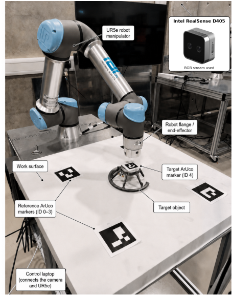
Fig. 2. Vision-guided workcell. An Intel RealSense D405 observes the surface from above; four reference markers bound the workspace and define the Board frame. Only the RGB stream is used. The UR5e approaches the target from above under a bounded two-stage motion.
