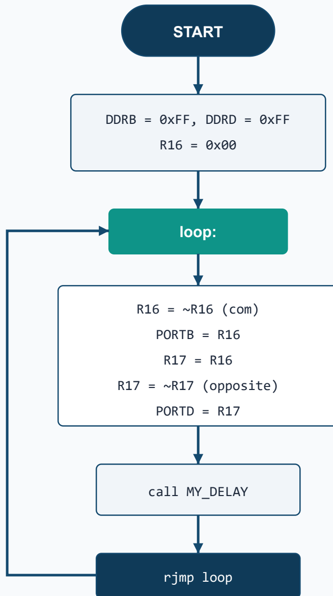
Flowchart 2: AssemblyBlink1_modified.asm
