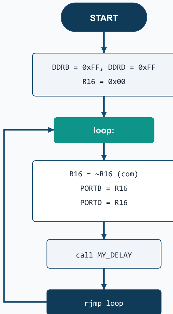
Flowchart 1: AssemblyBlink1.asm
