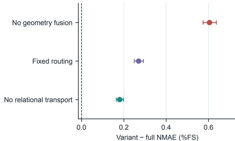
(b) Core ablation effects
