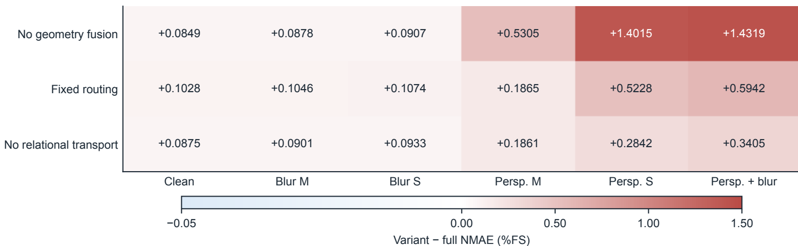
(c) Condition-wise core ablation effects
