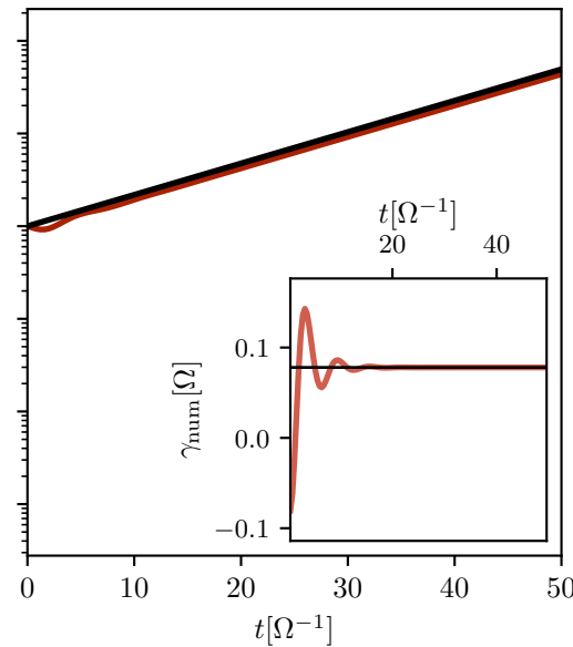
(c) \nu -slope driven instability
