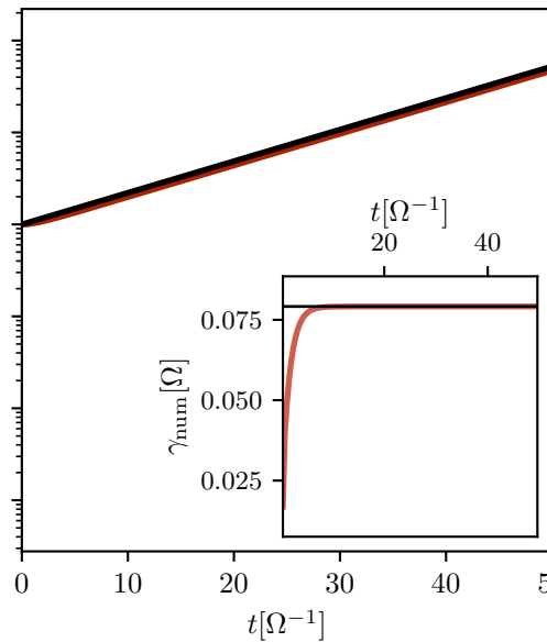
(b) D -slope driven instability
