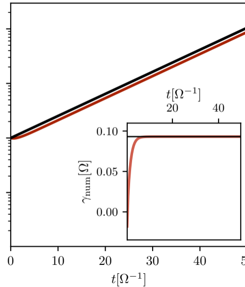
D -slope driven instability
