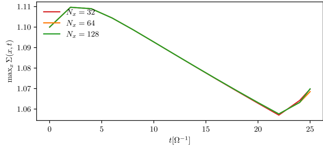
Neutral viscosity slope, native solver
