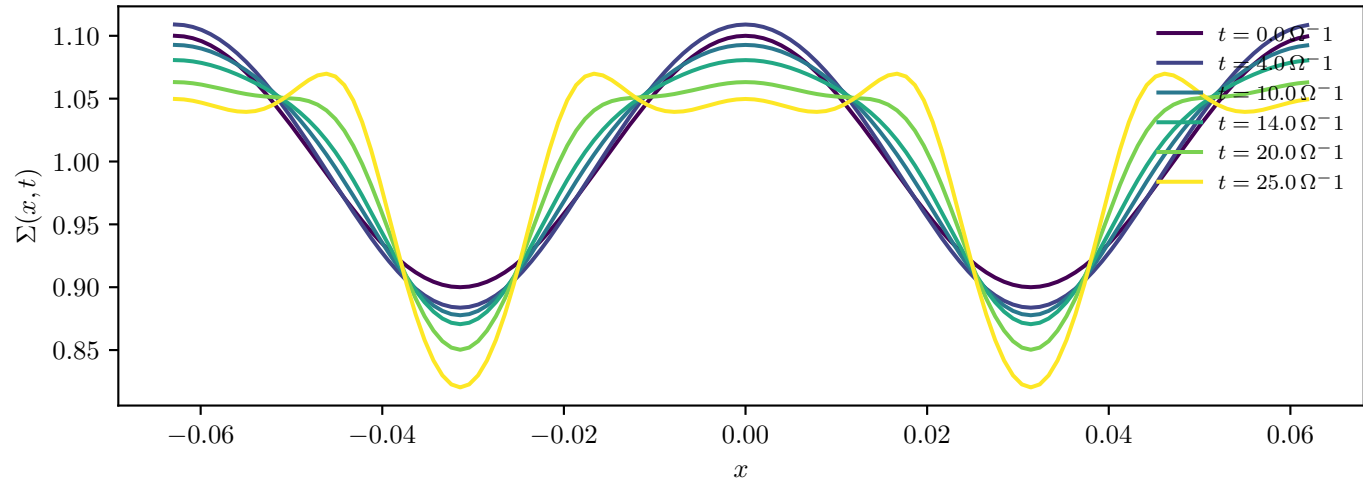
N_x = 128
