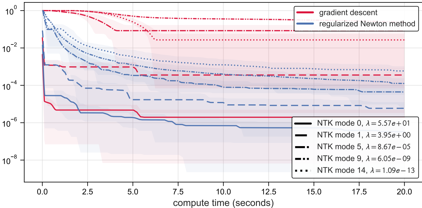
best relative NTK-mode error
