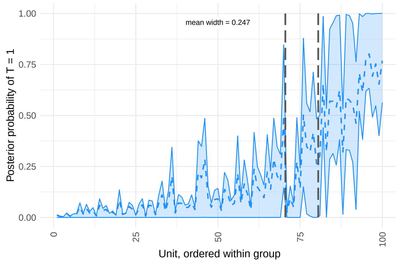
Covariates model
