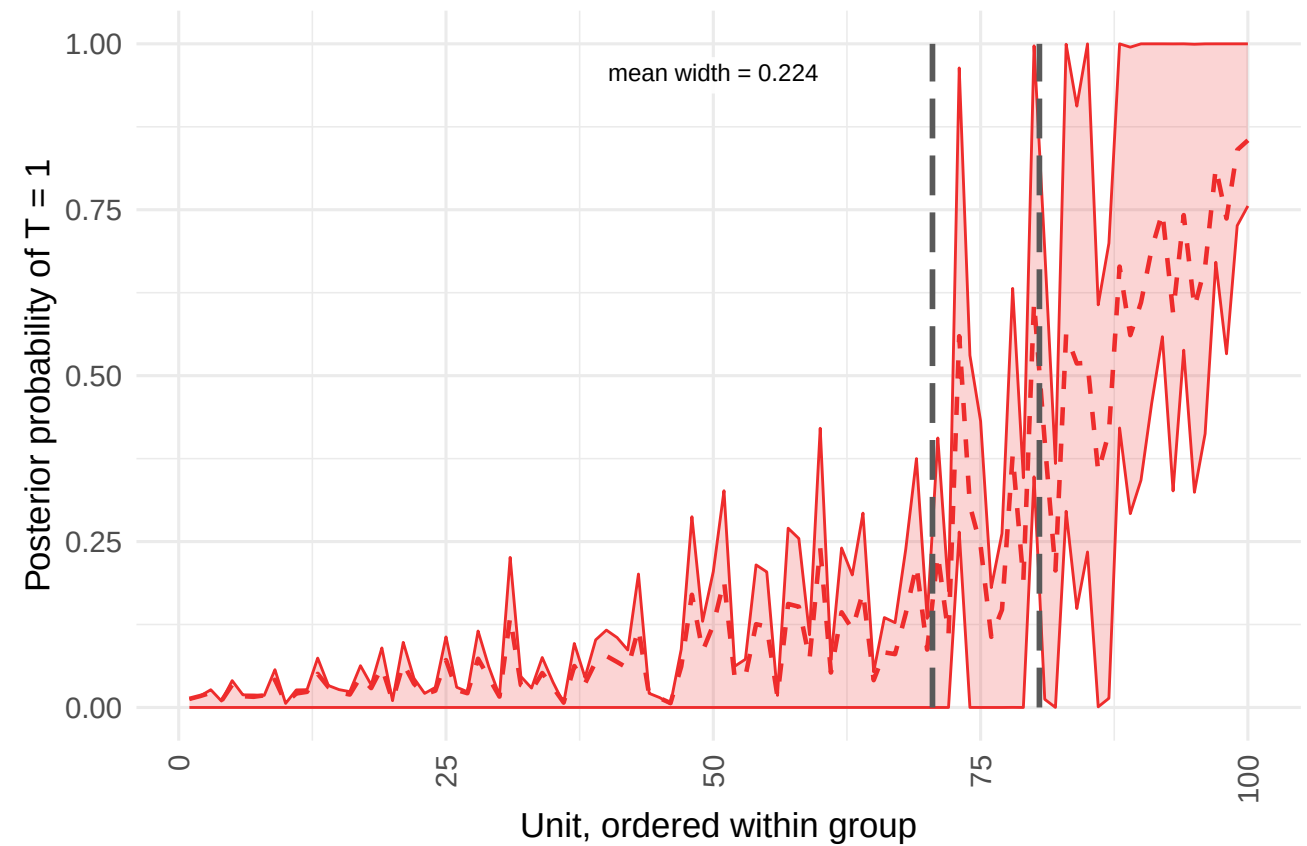
Network model
