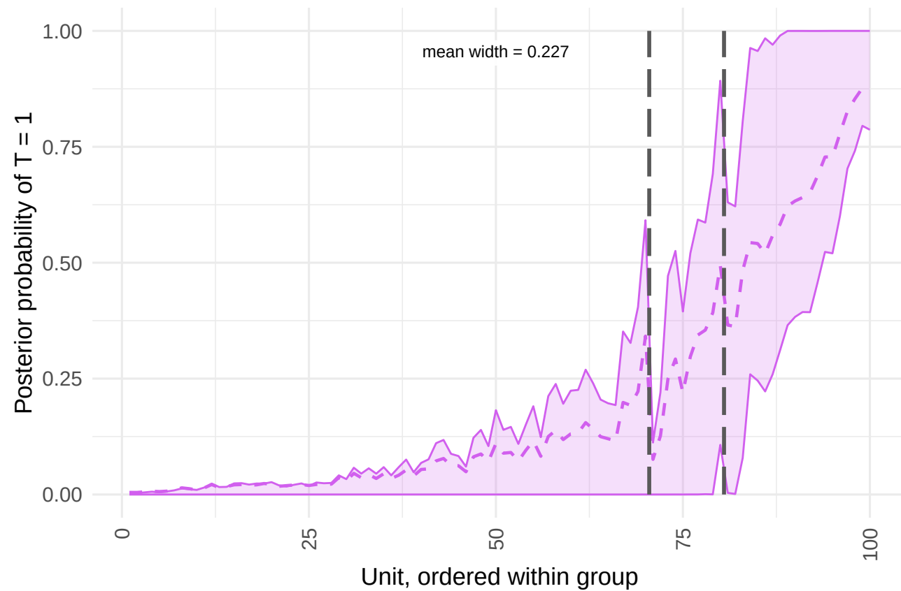
PoE model
