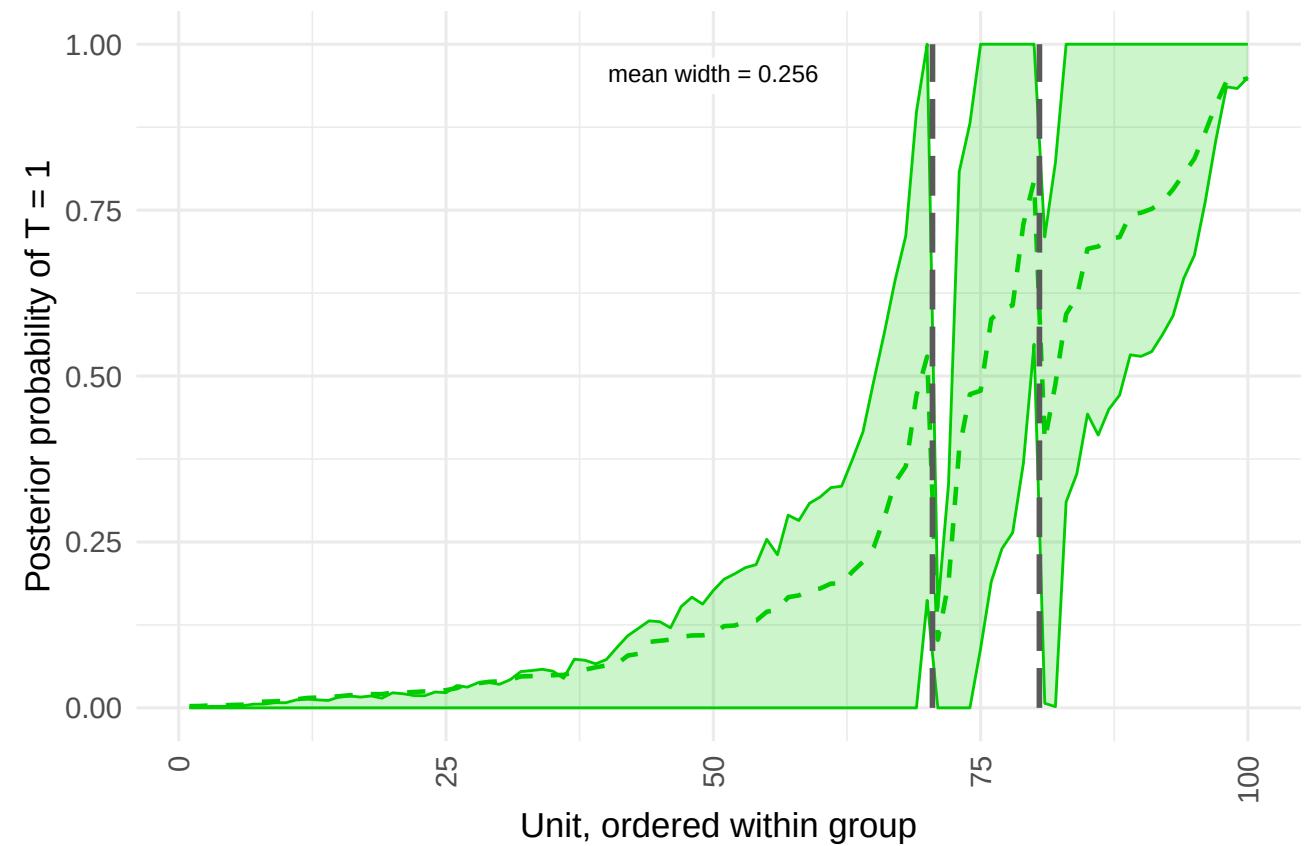
PU-PoE model
