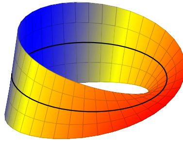
Figure 1.3: A parametric graph of a mobius strip.
