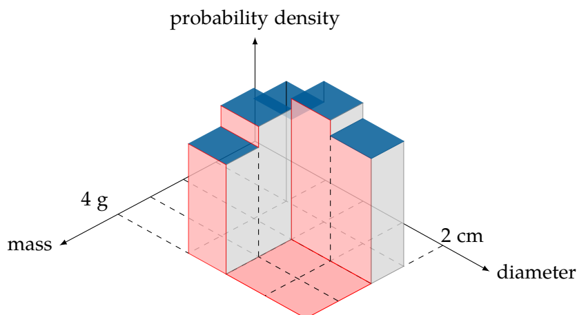
Figure 2.4: Reimann Sum
