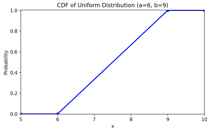
Figure 1.7: Cumulative distribution function for a uniform distribution between 6 and 9.
