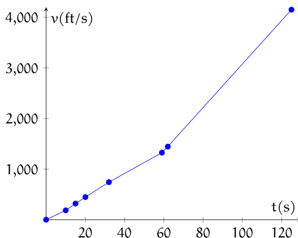
Figure 5.14: Plot of time, velocity data for the Endeavour
