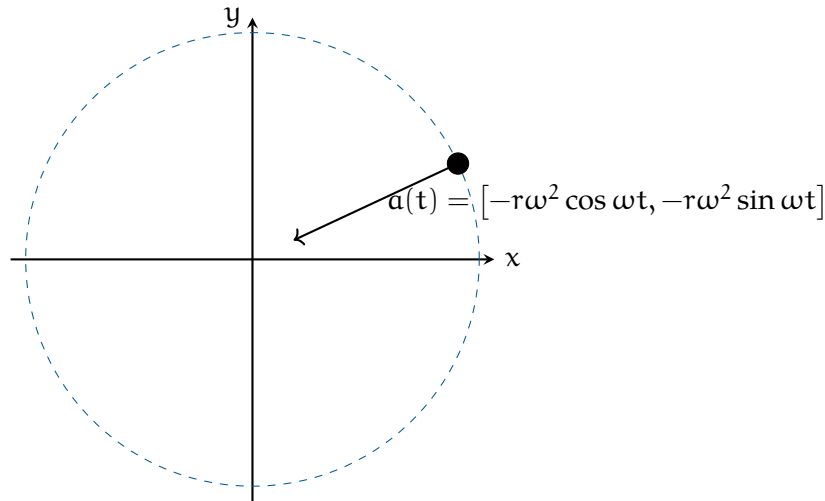
Figure 1.3: Acceleration vector of the particle in circular motion.
