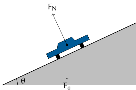
Figure 1.7: If there is no friction due to rain, then the only two forces acting on the car are gravity and the normal force.
