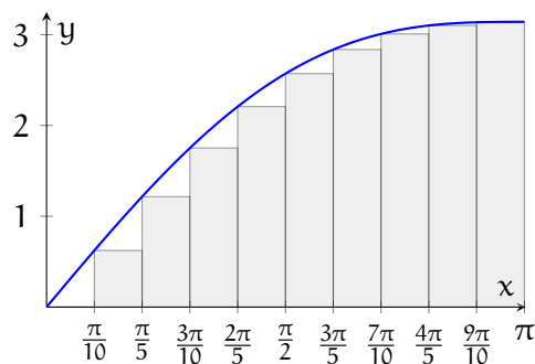
(a) Left-endpoint Riemann sum
