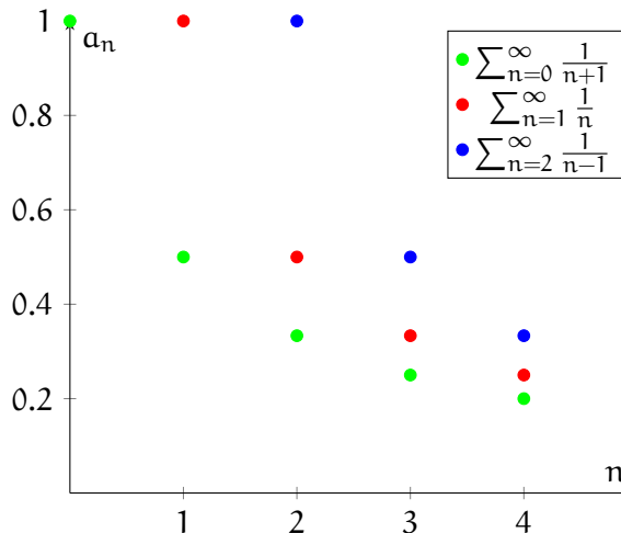
Figure 3.1: \sum_{n=0}^{\infty} \frac{1}{n+1} = \sum_{n=1}^{\infty} a_n = \sum_{n=2}^{\infty} = 1 + \frac{1}{2} + \frac{1}{3} + \dots
