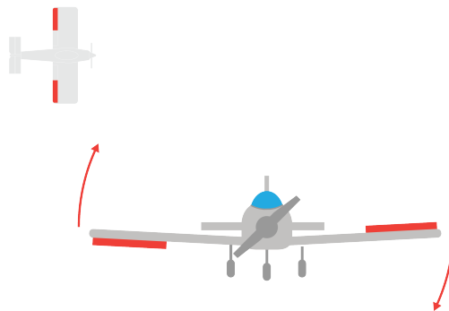
Figure 1.4: Aileron locations on the plane and their effect on roll.
