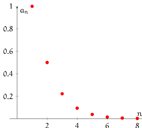
Figure 1.5: a_n = \frac{n!}{n^n}
