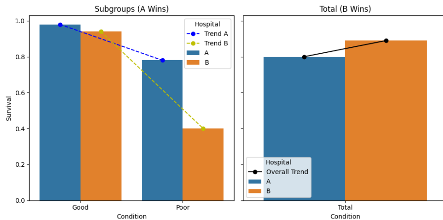
Figure 1.1: Simpson's Paradox: Subgroups vs. Total
