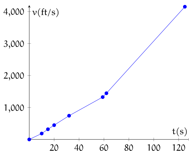
Figure 5.14: Plot of time, velocity data for the Endeavour
