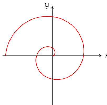
Figure 1.2: Archimedean spiral.
