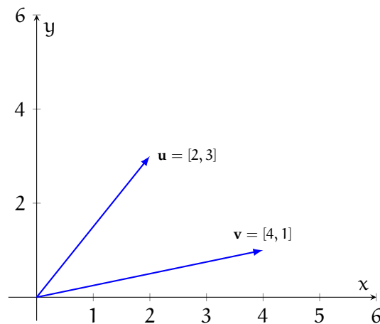
Figure 1.1: 2-dimensional vectors, u and v
