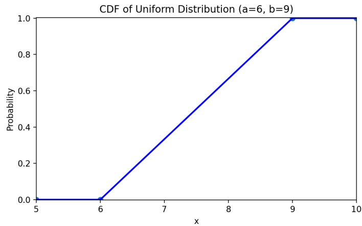
Figure 4.7: Cumulative distribution function for a uniform distribution between 6 and 9.
