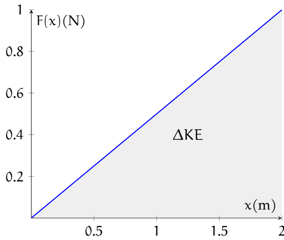
Figure 1.9: Force applied to a box over a distance; the shaded area represents the change in kinetic energy.
