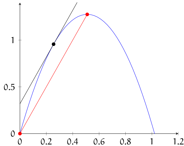
Figure 2.9: The height of a hammer tossed upwards at 5 \frac{\text{m}}{\text{s}}
