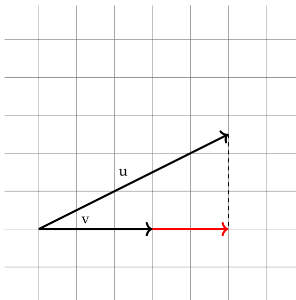
Figure 6.3: Projection vector extended beyond v .
