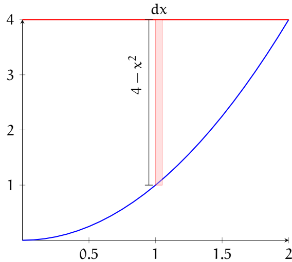
Figure 5.5: y = x^2 with a vertical cross-section
