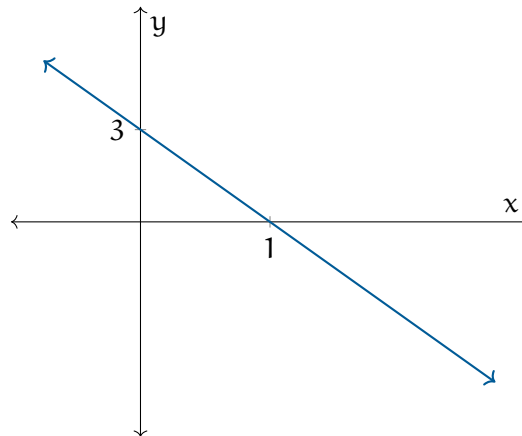
Figure 1.3: The resulting graph of f(x) = -3x + 3 .
