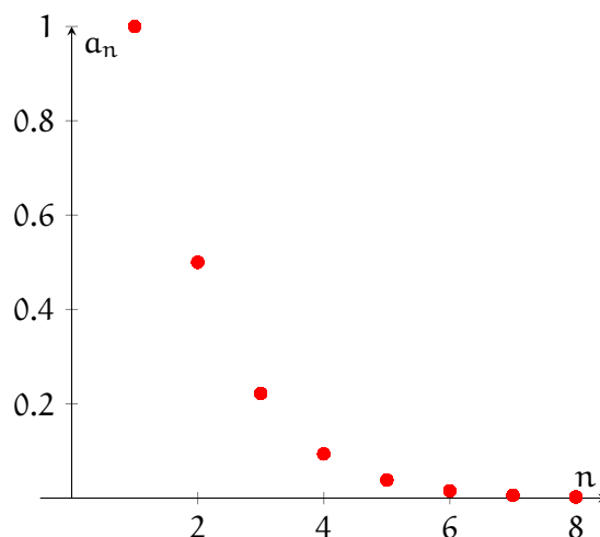
Figure 1.5: a_n = \frac{n!}{n^n}
