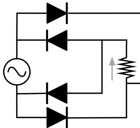
Figure 5.11: Full-wave Rectifier
