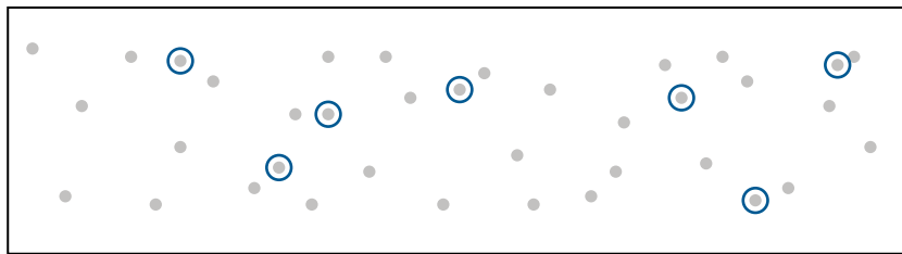
Figure 6.1: In simple random sampling, every individual in the population has an equal chance of being selected, and there is no grouping or pattern to who is chosen.
