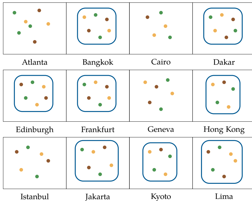
Figure 6.3: Each dot represents a customer and each color represents a different customer segment. Atlanta, Cairo, Geneva, and Istanbul were not selected. The other 8 cities were randomly selected as clusters, and every customer within each selected city becomes part of the sample.
