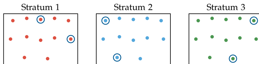
Figure 6.2: Each stratum is a single color, since members within a stratum share a characteristic. A small random sample (circled) is drawn from each stratum.
