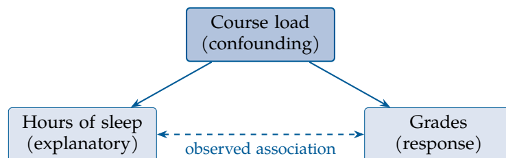
Figure 1.1: A confounding variable affects both the explanatory and response variables, so the observed association cannot be attributed to sleep alone.
