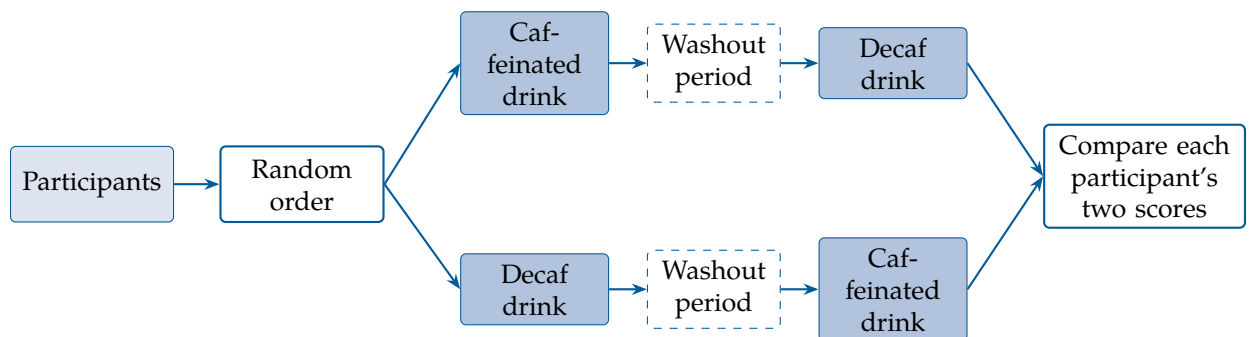
Figure 1.6: Schematic diagram of a matched-pairs design (repeated measures version).
