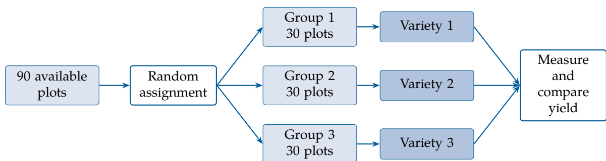
Figure 1.4: Schematic diagram of a completely randomized experiment.
