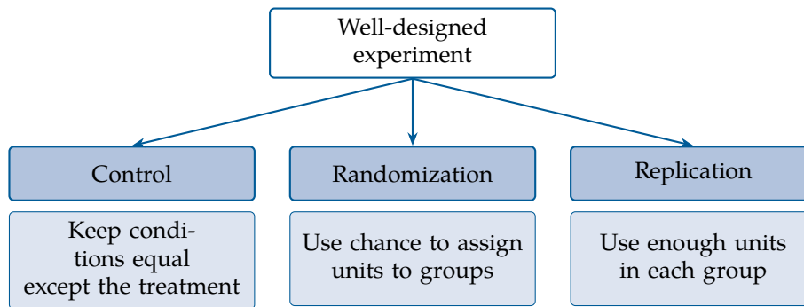
Figure 1.3: The three principles of experimental design.
