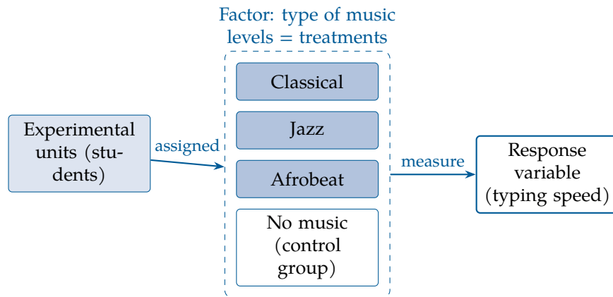
Figure 1.2: The parts of a one-factor experiment on background music and typing speed.
