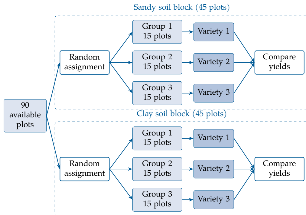
Figure 1.5: Schematic diagram of a randomized block design.
