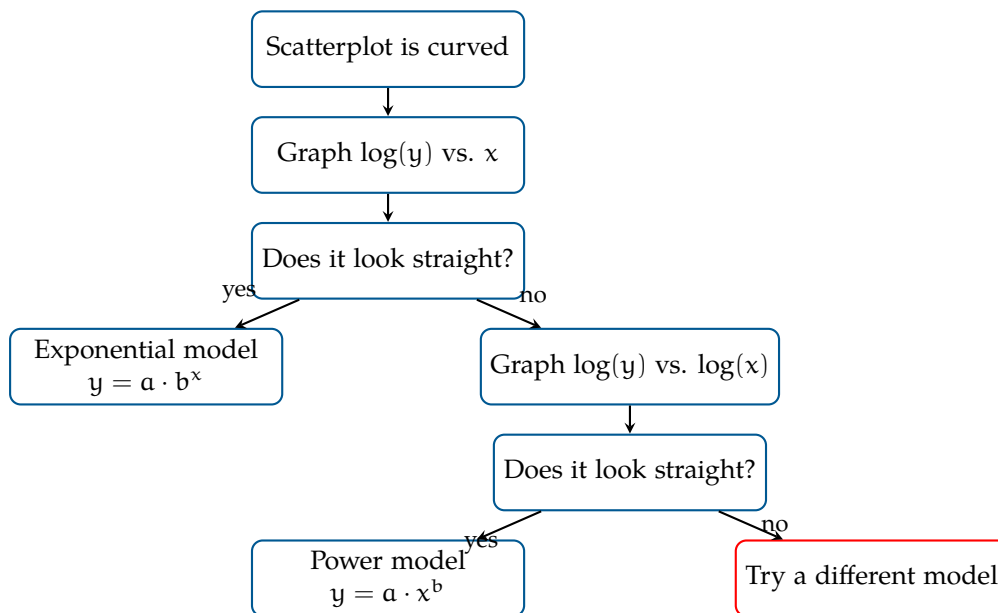
Figure 1.5: Deciding between an exponential and a power model.
