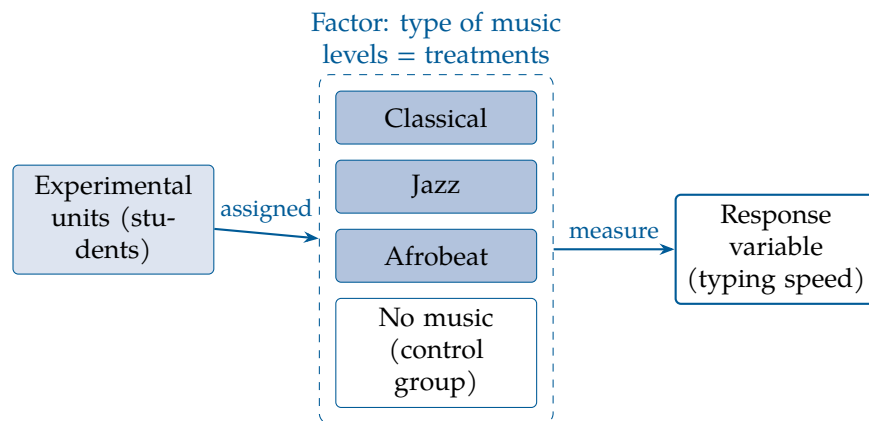
Figure 5.2: The parts of a one-factor experiment on background music and typing speed.
