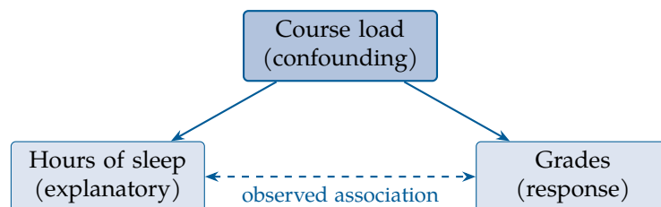
Figure 5.1: A confounding variable affects both the explanatory and response variables, so the observed association cannot be attributed to sleep alone.
