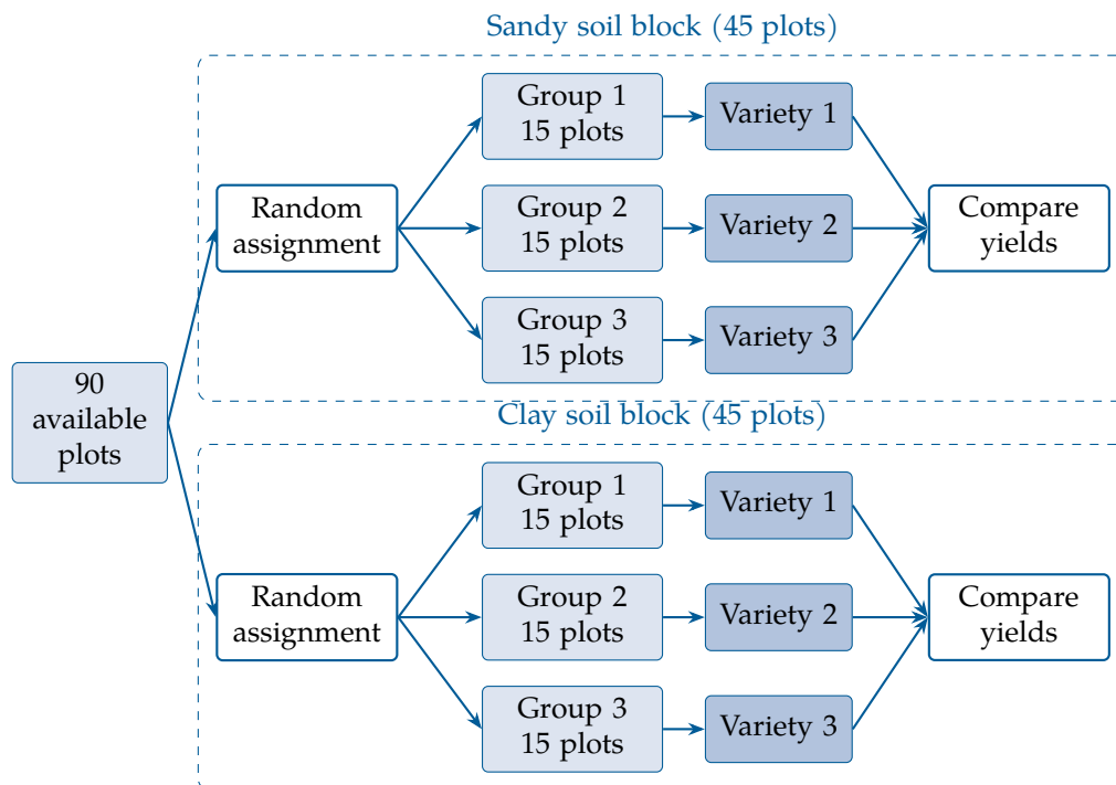
Figure 5.5: Schematic diagram of a randomized block design.
