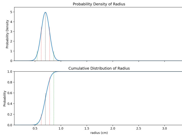
Figure 4.1: Ice sphere PDF and cumulative density function.
