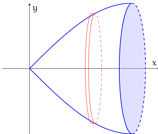
Figure 5.3: When rotated, the cross-section becomes a cylinder with radius \sin x and width dx , which has a total volume of \pi \sin^2 x dx
