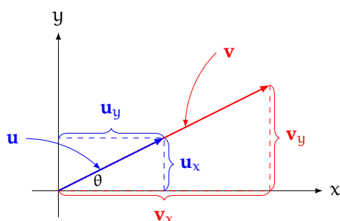
Figure 5.9: \mathbf{u} is a unit vector in the same direction as \mathbf{v}
