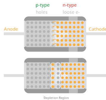
Figure 6.6: The depletion region in a diode
