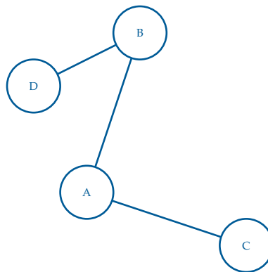
Figure 6.1: A simple (undirected unweighted) graph used to make an adjacency list and adjacency matrix.
