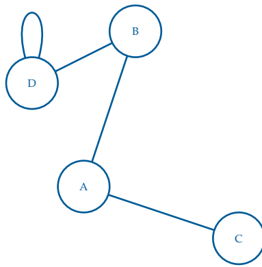
Figure 6.2: A simple graph with an added loop on vertex D.
