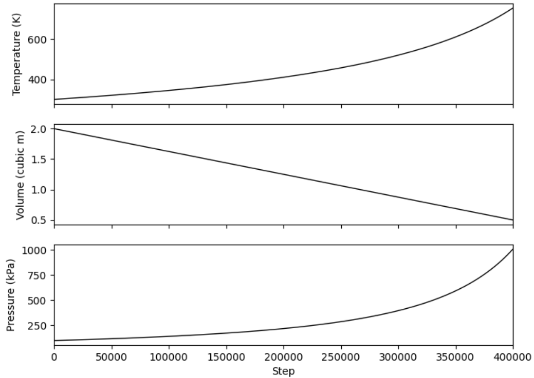
Figure 2.2: Chunk plots of temperatures every 400 steps.
