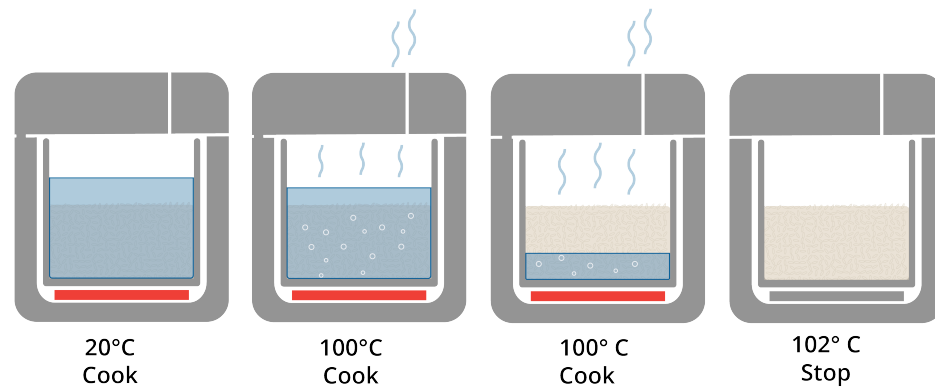
Figure 3.3: The various phases of a rice cooker.
