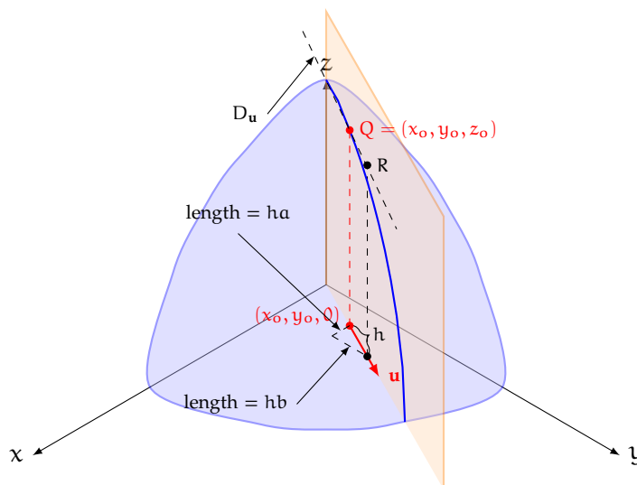
Figure 5.8: A second point, R, along \mathbf{u} is h units away along \mathbf{u}
