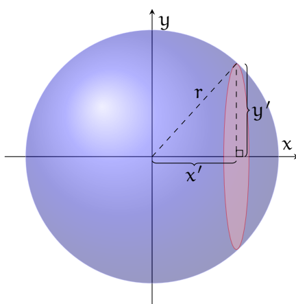
Figure 5.1: A vertical cross-section of a sphere
