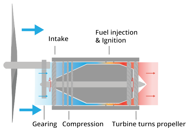
Figure 1.9: Cross section of a turboprop
