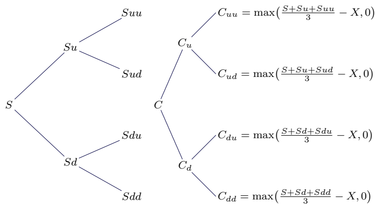
Figure 10.8.: Two periods of an average-rate call. The stock tree on the left recombines ( Sud = Sdu ); the pricing tree on the right does not, since C_{ud} \neq C_{du} in general. With C_u = [pC_{uu} + (1-p)C_{ud}]/e^{\hat{r}} and similarly for C_d and C , the pricing tree grows exponentially.
