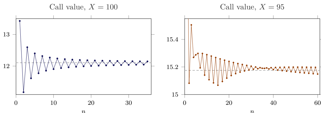
Figure 8.12.: CRR binomial call values against the number of periods n , with S = 100 , r = 8\% , \sigma = 0.2 , \tau = 1 . Dashed: the Black–Scholes values 12.1058 (left) and 15.1749 (right). The value at n = 1 on the right (16.46) is off the scale.
