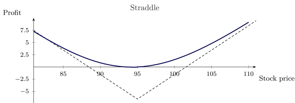
Figure 6.11.: Profit of a straddle with X = 95 , bought when S = 95 one month before expiration for C + P = 6.56 . Dashed: the V-shaped profit at expiration, (6.6) less the two premiums, with break-evens at X \pm (C + P) . Solid: profit at entry. The solid curve rises above the dashed one at both ends and sits above its vertex — a straddle held rather than exercised loses only time value, which is why the position is a bet on volatility and not on price.
