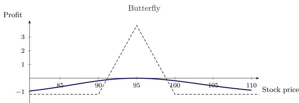
Figure 6.10.: Profit of a butterfly spread with X_L = 90 , X_M = 95 , X_H = 100 , entered when S = 95 one month before expiration at a cost of 1.17. Dashed: the tent-shaped profit at expiration, positive only between X_L and X_H . Solid: profit at entry, which is nearly flat — with a month of time value still in the options, the market has not yet decided the bet.
