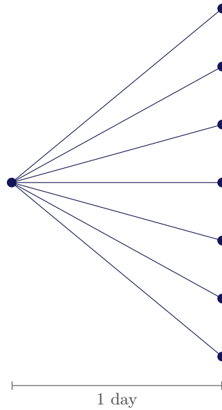
Figure 10.7.: A heptanomial tree: 6 periods per day, intraday nodes removed. The seven successors are the end-of-day prices Su^{6-2j} , j = 0, \dots, 6 .
