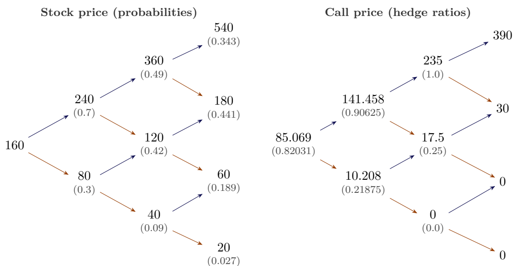
Figure 8.7.: Example 8.12.1. Left: the binomial process for the stock, with the risk-neutral probability of reaching each node. Right: the call values by backward induction, with the delta (8.3) at each node.
