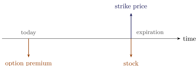
Figure 6.2.: Cash flows of a long put — Figure 6.1 with the roles of stock and strike price interchanged.
