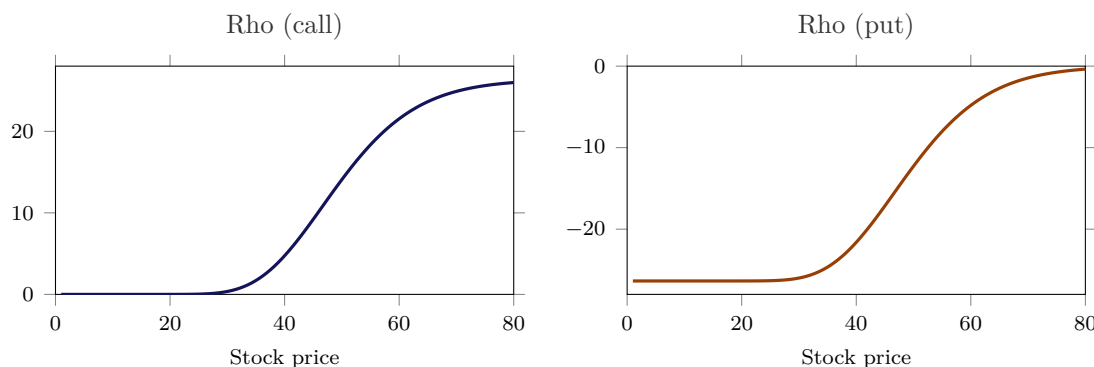
Figure 9.5.: Rho with X = 50 , \sigma = 30\% , r = 8\% , \tau = 201 days. Deep in the money the call's rho tends to X\tau e^{-r\tau} \approx 26 , the rate sensitivity of the bond Xe^{-r\tau} it effectively shorts.
