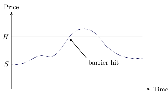
Figure 10.2.: A price path that touches the barrier H : a knock-out option on this path is dead from that moment on, and a knock-in option comes alive — even though the path ends below H .
