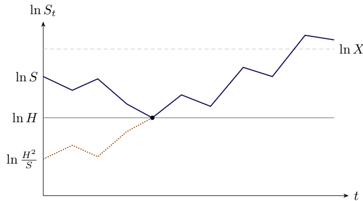
Figure 10.4.: The reflection principle. Every path from \ln S that touches \ln H and ends above \ln X (solid) pairs with the path from \ln(H^2/S) that mirrors it up to the first touch (dotted) and coincides with it afterwards.
