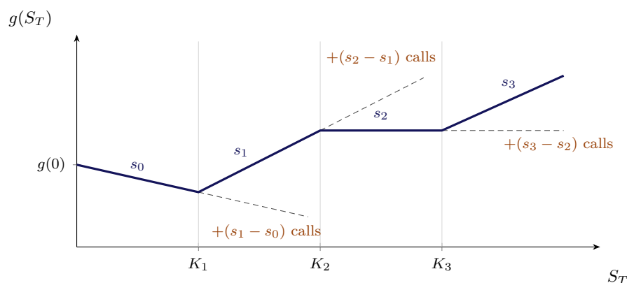
Figure 7.2.: A piecewise linear payoff with kinks K_1, K_2, K_3 and slopes s_0, \dots, s_3 . The bond and the stock produce the first segment; at each kink the dashed line is where the previous segment would have gone, and the calls struck there (labelled in red) bend it onto the next slope.
