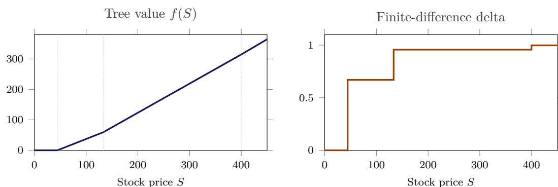
Figure 9.7.: The three-period call of Example 8.12.1 as a function of the initial price S (with u, d, R, X fixed). It is piecewise linear with kinks at S = X/(u^j d^{3-j}) (dotted), so a small-step finite-difference delta is a ladder, and the finite-difference gamma is 0 almost everywhere and huge at the kinks.
