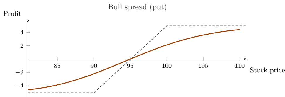
Figure 6.8.: Profit of a bull put spread with X_L = 90 , X_H = 100 , entered when S = 95 one month before expiration for a net credit of P_H - P_L = 4.94 . Dashed: profit at expiration. Solid: profit at the moment of entry as the stock price varies. The shape is that of Figure 6.7; the plateaus sit at 4.94 and -5.06 instead of 4.98 and -5.02 .
