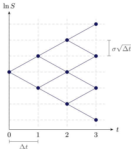
Figure 8.11.: The CRR tree in logarithmic coordinates: every move is \pm\sigma\sqrt{\Delta t} , and since ud = 1 the tree is symmetric about the starting level.
