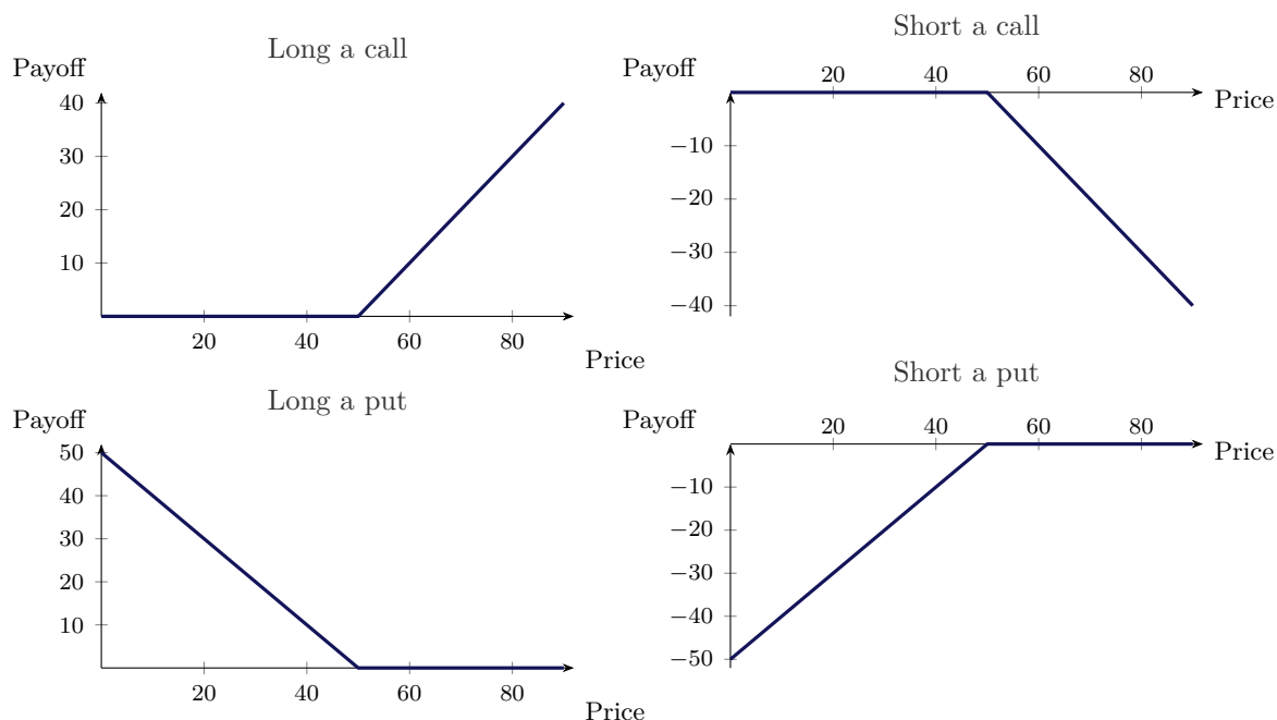
Figure 6.3.: Payoffs at expiration of the four elementary option positions, with strike X = 50 . These are payoffs, not profits: the premium has not been subtracted. The kink always sits at S = X . Note the asymmetry in the writer's risk — a short call has unbounded loss as S \rightarrow \infty , whereas a short put loses at most X , since the stock cannot fall below zero.
