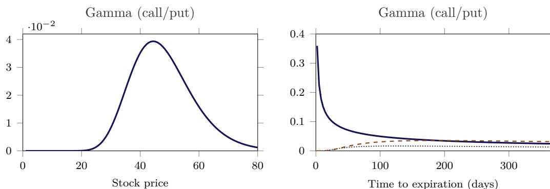
Figure 9.3.: Gamma with X = 50 , \sigma = 30\% , r = 8\% ; right: S = 60 (dotted), 50 (solid), 40 (dashed). The at-the-money gamma grows like 1/\sqrt{\tau} as \tau \rightarrow 0 ; the others die out.
