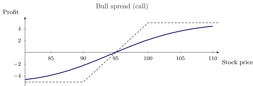
Figure 6.7.: Profit of a bull call spread with X_L = 90 , X_H = 100 , entered when S = 95 one month before expiration for a net debit of C_L - C_H = 5.02 . Dashed: profit at expiration, a ramp clipped at both ends. Solid: profit at the moment of entry as the stock price varies. The maximum profit 4.98 and the maximum loss 5.02 are the two dashed plateaus.
