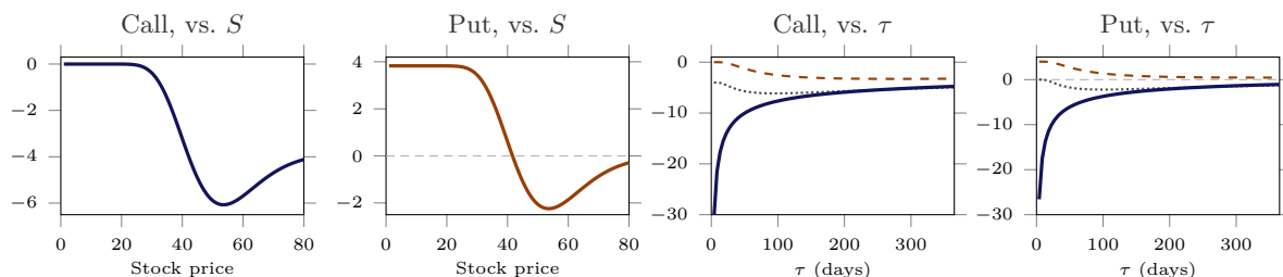
Figure 9.2.: Theta (per year), X = 50 , \sigma = 30\% , r = 8\% . Left two: \tau = 201 days. Right two: S = 60 (dotted), 50 (solid), 40 (dashed). The call's theta is always negative; the put's turns positive deep in the money, tending to rXe^{-r\tau} . At the money the theta plunges as \tau \rightarrow 0 .
