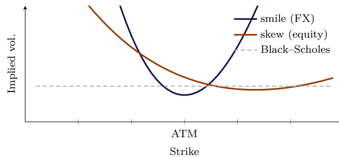
Figure 8.13.: Schematic shapes of implied volatility against strike. The slides show real data for TXO calls on September 25, 2015 (TAIEX closed at 8132), where implied volatility ranged from about 14% to 24% across strikes and maturities.
