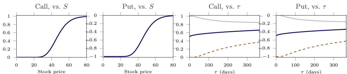
Figure 9.1.: Call and put deltas, X = 50 , \sigma = 30\% , r = 8\% . Left two: \tau = 201 days. Right two: S = 60 (dotted), 50 (solid), 40 (dashed). Each put curve is the call curve shifted down by 1, by (9.3).
