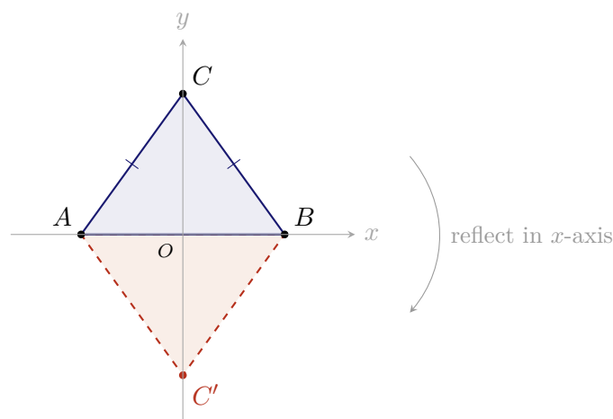
Figure 1.2.: The isosceles triangle \triangle ABC is symmetric about the y -axis; its reflection in the x -axis (dashed) is visibly different.
