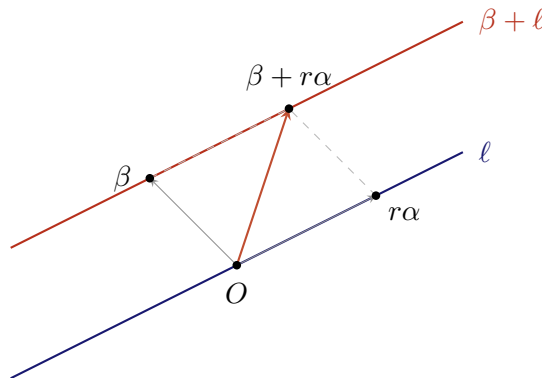
Figure 1.4.: The coset \beta + \ell is the line through \beta parallel to \ell .
