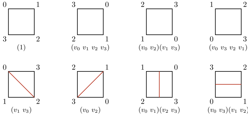
Figure 1.5.: The dihedral group D_8 acting on the vertices of a square. Label i marks where the vertex v_i is sent; the top row shows the rotations, the bottom row the reflections (with their axes).
