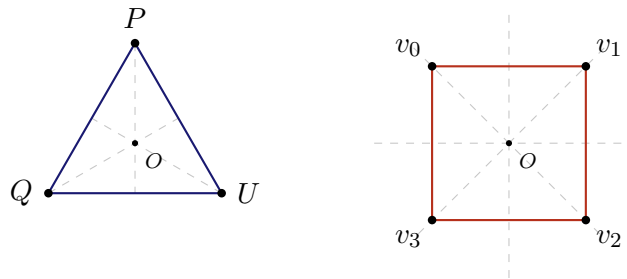
Figure 1.3.: Reflection axes of a regular 3-gon and a regular 4-gon.
