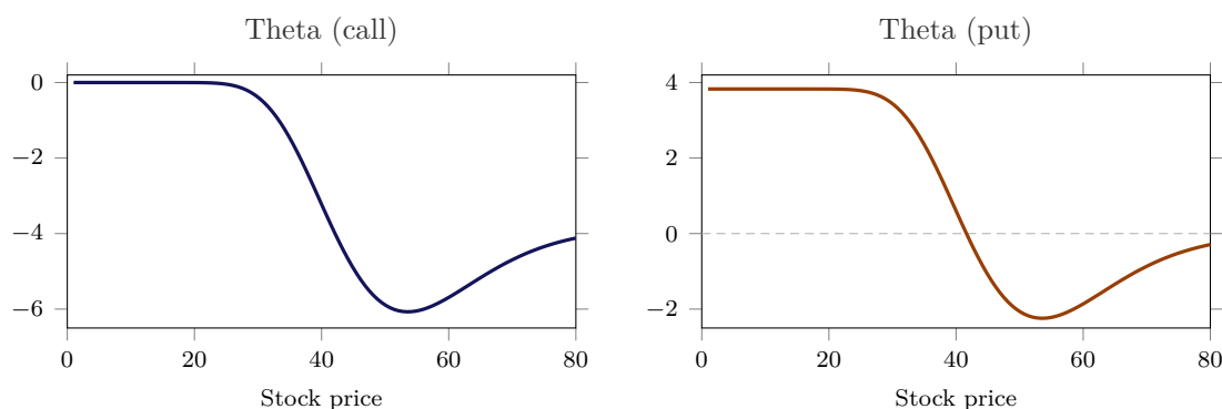
Figure 9.2.: Theta (per year) with X = 50 , \sigma = 30\% , r = 8\% , \tau = 201 days. The call's is always negative and most negative near the money; the put's turns positive deep in the money, where it tends to rXe^{-r\tau} .
