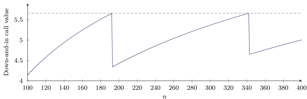
Figure 10.6.: CRR binomial values of the down-and-in call of Figure 10.3 ( S = 95 , X = 100 , H = 90 , r = 10\% , \sigma = 25\% , \tau = 1 ), computed by in-out parity, for n = 100, \dots, 400 . Dashed: the analytical value 5.6605. Each jump down happens when the effective barrier moves to the next lattice level; in between the value creeps up with an odd-even wobble. Cf. Lyuu (1998).
