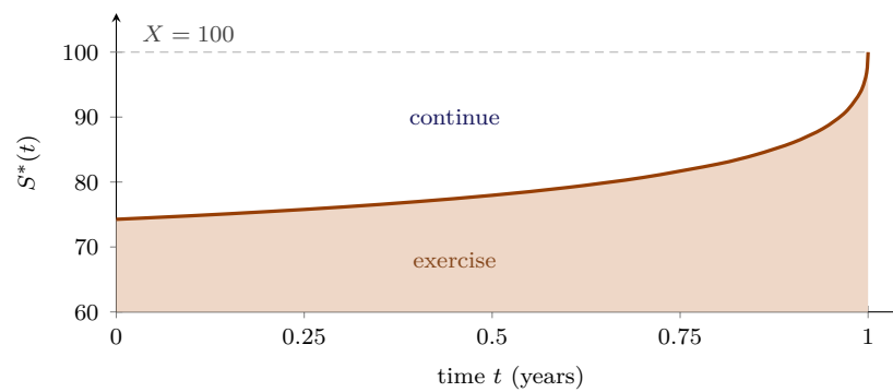
Figure 8.15.: Exercise boundary of an American put with X = 100 , r = 8\% , \sigma = 30\% , expiring at t = 1 , computed by Algorithm 8.4 with 600 periods and bisection on S . Below the curve, immediate exercise is optimal. The boundary rises to X at expiration.
