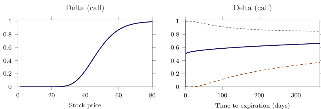
Figure 9.1.: Call delta with X = 50 , \sigma = 30\% , r = 8\% ; left with \tau = 201 days, right against \tau for S = 60 (dotted, in the money), S = 50 (solid, at the money) and S = 40 (dashed, out of the money). The put delta is the same picture shifted down by 1, by (9.3).
